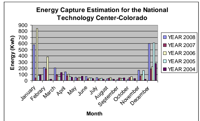
Figure 1: Energy Capture Estimation for the National Technology Center - Colorado using weibull distribution
