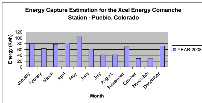
Figure 3: Energy Capture Estimation for the Xcel Energy Comanche Station- Pueblo, Colorado using weibull distribution
