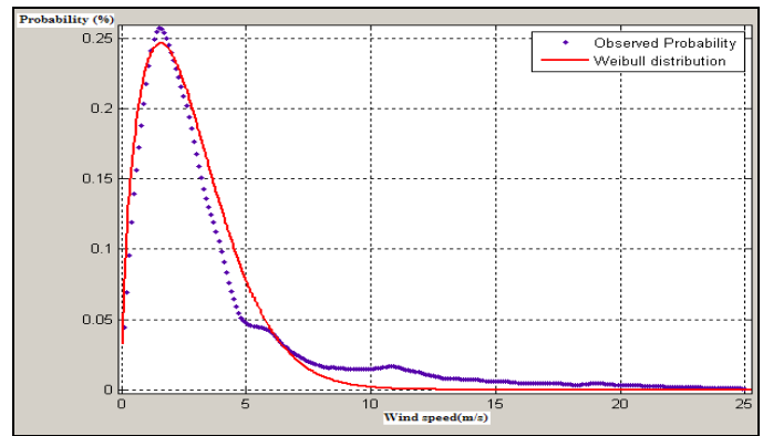
Figure 4: Probability plot and Weibull distribution curve fitting of wind data January 2007- National Technology Center-Colorado
