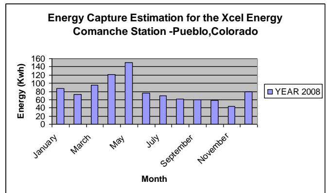
Figure 6: Energy Capture Estimation for the Xcel Energy Comanche Station- Pueblo, Colorado using computational method
