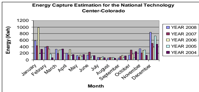
Figure 4: Energy Capture Estimation for the National Technology Center – Colorado using computational method
