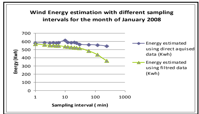
Figure 7: Wind Energy estimation with different sampling intervals for the month of January 2008 (National Wind Technology Center-Colorado) using filtered and no filtered wind speed Data
