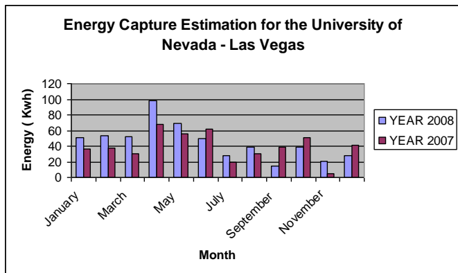
Figure 5: Energy Capture Estimation for the University of Nevada – Las Vegas using computational method
